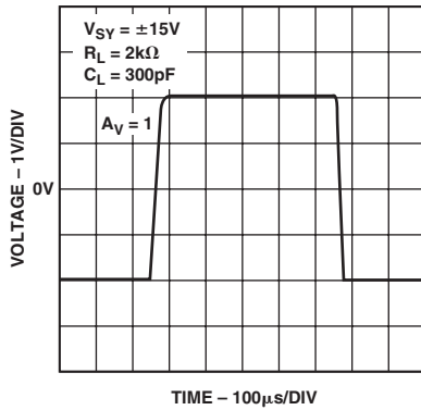
TPC 22. Large Signal Transient Response
